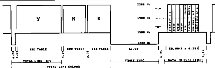
Fig. 1 BASIC TIMING DIAGRAM (All times in \mu s.)
